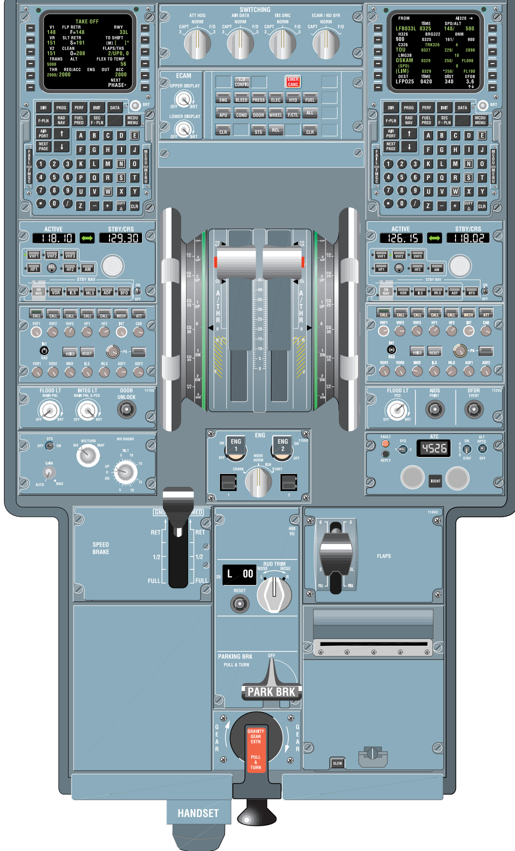
Airbus A320 Pedestal Panel
